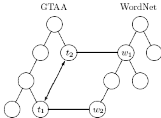
Figure 1: Using the anchoring to WordNet to infer relations within the GTAA.
